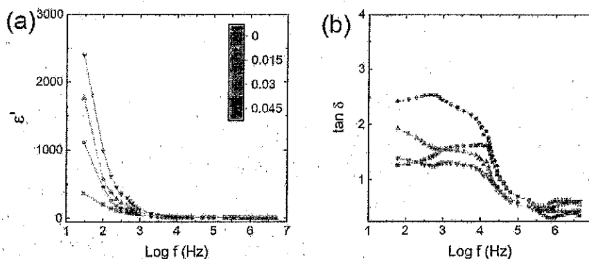
Fig. 10 \text{Co}_{0.4}\text{Cu}_{0.1}\text{Zn}_{0.5}\text{Dy}_x\text{Fe}_{2-x}\text{O}_4 dielectric parameters, each as a function of logarithm of frequency (f). (a) Real part of dielectric constant ( \epsilon' ) and (b) dielectric loss tangent ( \tan \delta ).
